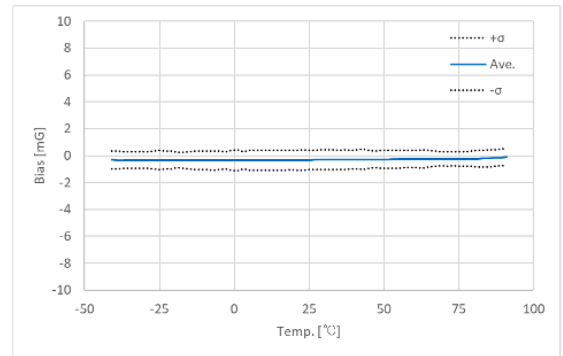
Figure 3.5 Accelerometer Bias vs. Temperature Characteristic
