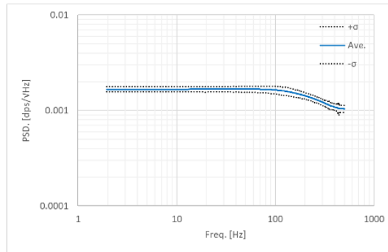
Figure 3.3 Gyro Noise Frequency Characteristic
