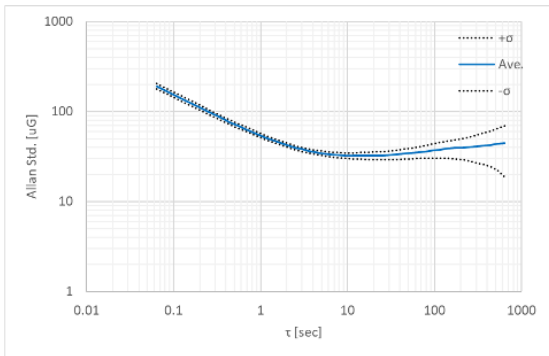
Figure 3.4 Accelerometer Allan Variance Characteristic
