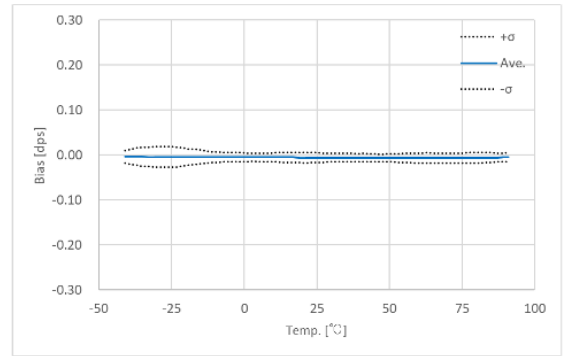
Figure 3.2 Gyro Bias vs. Temperature Characteristic
