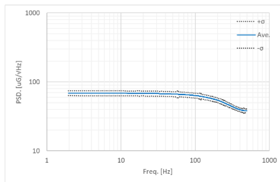
Figure 3.6 Accelerometer Noise Frequency Characteristic
