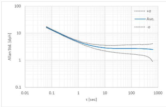
Figure 3.1 Gyro Allan Variance Characteristic
