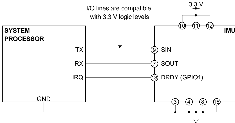
Figure 4.2 UART Connection
