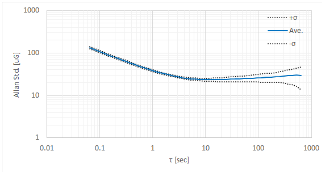
Figure 3.4 Accelerometer Allan Variance Characteristic
