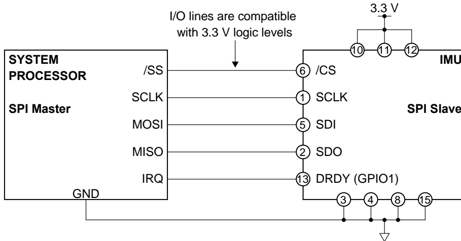
Figure 4.1 SPI Connection
