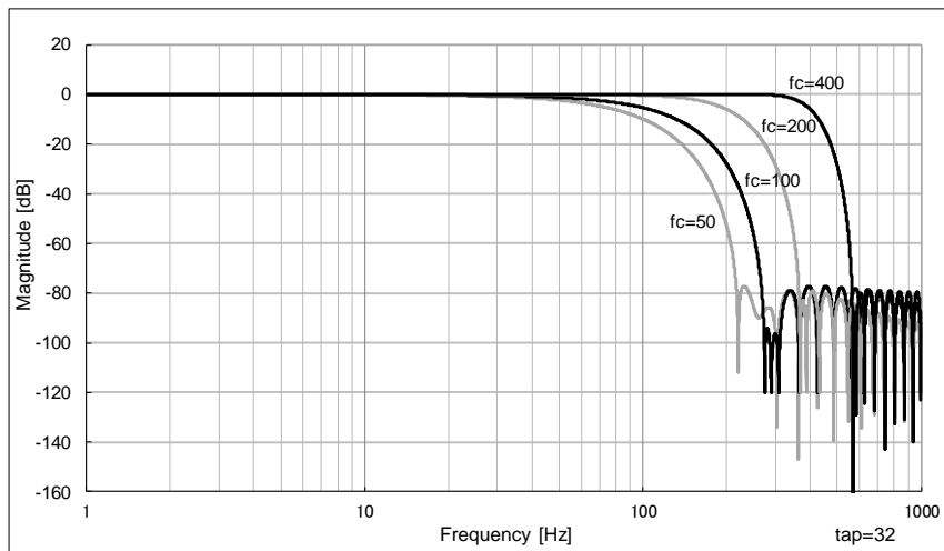
Figure 4.13 FIR Kaiser Filter Typical Characteristic 1
