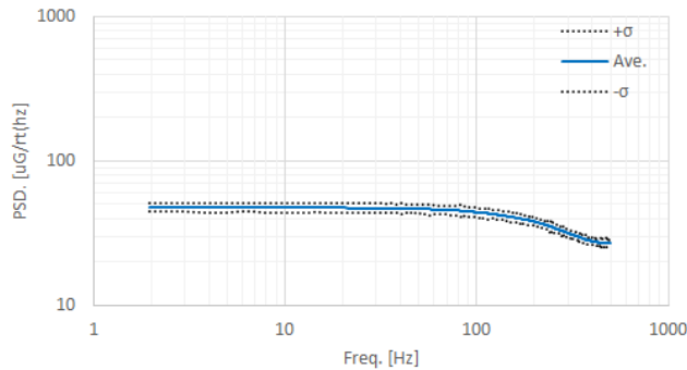
Figure 3.6 Accelerometer Noise Frequency Characteristic
