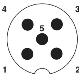
Terminal Layout
