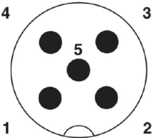
Terminal Layout
