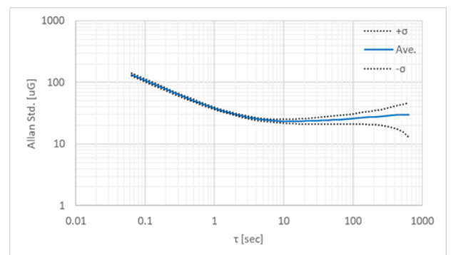
Accelerometer Allan Variance Characteristic
